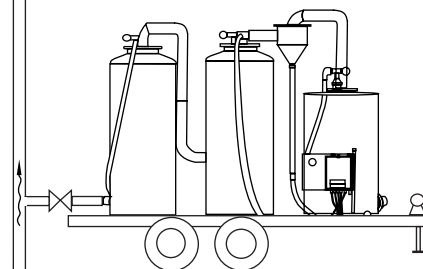
PACKED TOWER RECIRCULATING CAUSTIC SCRUBBER W/EMTOS OR CARBON POLISH
