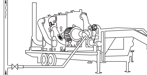
MULTI-CHAMBERED HIGH-VOLUME LIQUID/MEDIA ABSORBER
